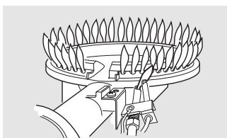
Figure A: Main burner and pilot flame pattern. (Cast iron burner)
