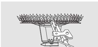
Figure B: Main burner and pilot flame pattern. (Sheet metal burner)
